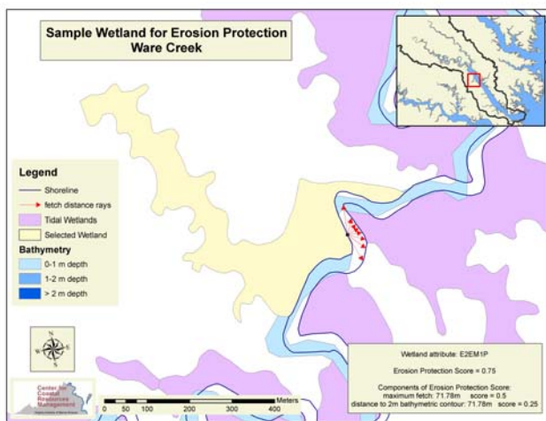
Figure 9. Erosion score for wetland polygon #1256, middle York River.
