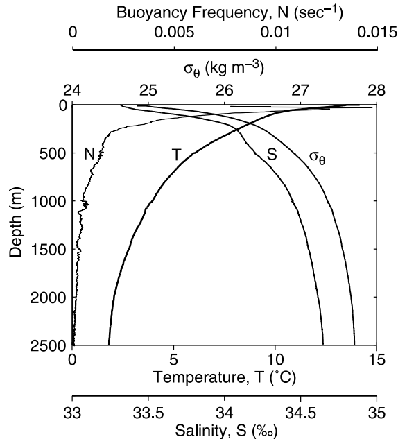
Fig. 2. Temperature and salinity profiles used for model initialization, and the corresponding density ( \sigma_\theta ) and buoyancy frequency ( N ) profiles.
