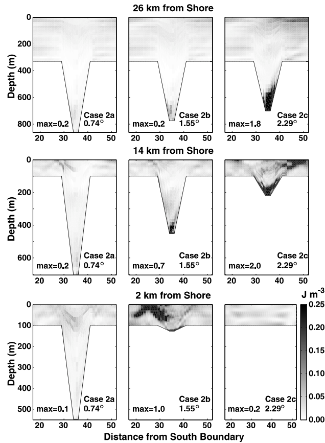
Fig. 15. Case 2 energy density, E ( \text{J m}^{-3} ), cross-canyon sections 26 km (upper), 14 km (middle), and 2 km (lower) from the eastern boundary.
