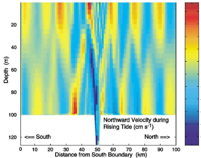
Fig. 12. Along shelf section of v 2 km from model eastern boundary showing evolution of the internal tide from beam-like near the canyon rims to first mode-like further away.
