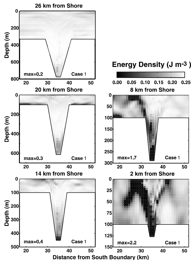
Fig. 9. Case 1 cross-canyon sections of energy density, E . Note that a different vertical scale is used for each section.
