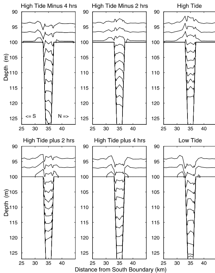
Fig. 11. Cross-canyon density sections 2 km from the eastern boundary at six times during the tidal cycle. The in situ densities are contoured in intervals of 0.03 \text{ kg m}^{-3} , and range from 26.335 to 26.635 \text{ kg m}^{-3} .
