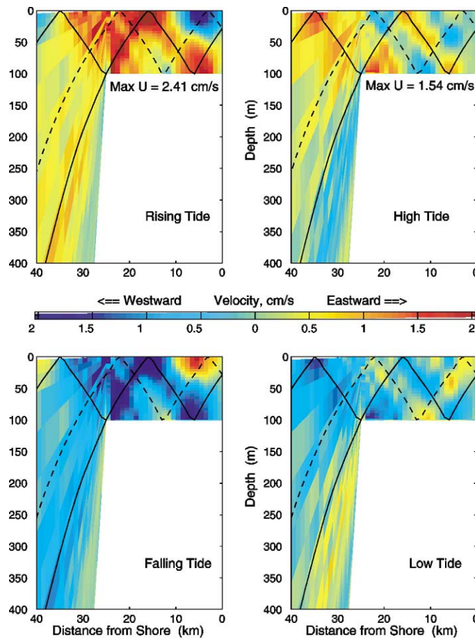
Fig. 4. Cross-shelf sections of u at four times during the semidiurnal tidal cycle, as indicated by the stage of the sea level, together with characteristics emanating from the shelf break (—) and reflecting from the coastal boundary (---). Note the 180^\circ phase shift in horizontal velocity after reflection from the vertical boundary.
