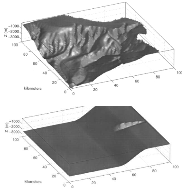
Fig. 1. Monterey Bay bathymetry and a sample model bathymetry that incorporates a relatively narrow shelf, a steep ( 7^\circ ) continental slope, a deep basin, and a canyon head lying close to shore.
