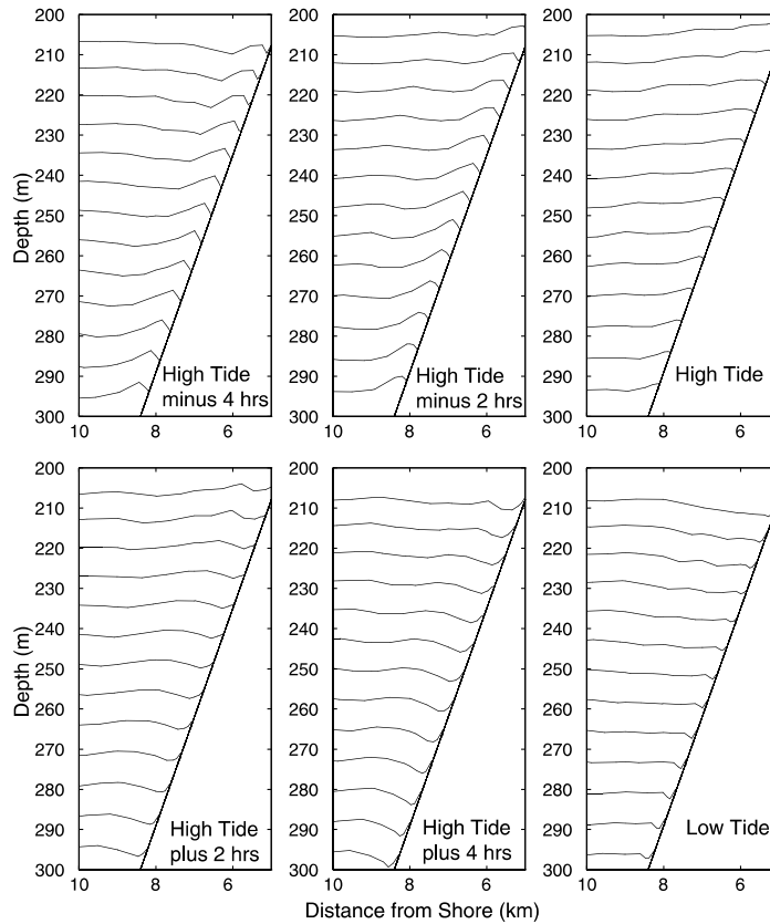
Fig. 7. Density sections along the critically sloping portion of the model canyon at six times during the tidal cycle. In situ densities ranging from 1027.35 to 1027.95 \text{ kg m}^{-3} are contoured at intervals of 0.05 \text{ kg m}^{-3} .
