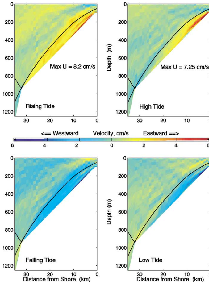
Fig. 6. Along-canyon sections of u at four times during the semidiurnal tidal cycle, as indicated by the stage of the sea level, together with characteristics emanating from the shelf break (—). Note that the velocity scale in Fig. 6 has been expanded to \pm 6 \text{ cm s}^{-1} , versus the \pm 2 \text{ cm s}^{-1} scale used for the shelf currents in Fig. 4.
