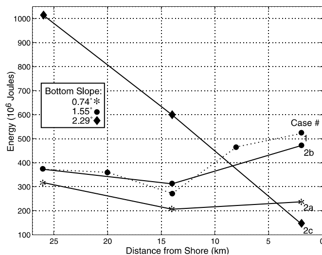
Fig. 10. Total energy in three cross-canyon sections (positions indicated in Fig. 5) for model case 2 (Fig. 15). Total energy values are shown for two additional cross-canyon sections for case 1 (Fig. 9). Each value represents energy integrated over a volume 31 km alongshore by 1 km cross-shore by depth.
