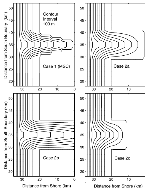
Fig. 13. Bathymetry for model cases 1 and 2, as described in Table 1, are shown. The contour interval is 100 m.
