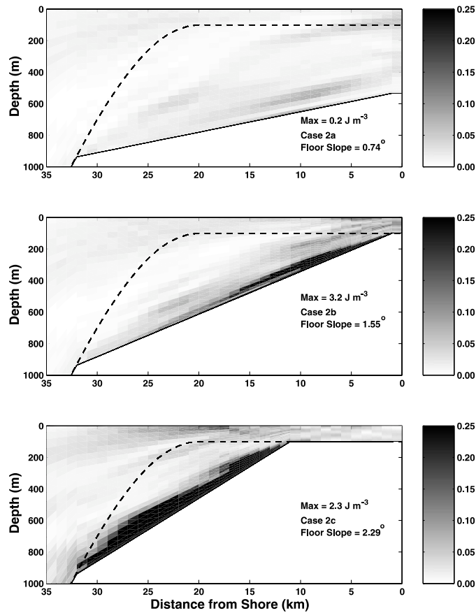
Fig. 14. Case 2 energy density, E ( \text{J m}^{-3} ), along-canyon sections. The canyon floor slope for each case is indicated. The canyon is 11 km wide at the rim and 3 km wide at the floor in all three studies. Bottom profiles for the continental shelf and slope adjacent to the canyon (---) are also shown.
