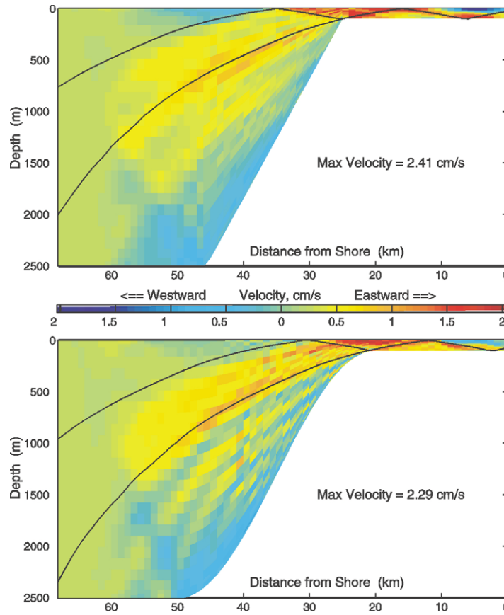
Fig. 3. Cross-shelf sections of u during rising sea level for a sharp (upper) and cosine-shaped (lower) continental shelf break together with characteristics (—) from the linear internal wave dispersion relation including rotation effects.
