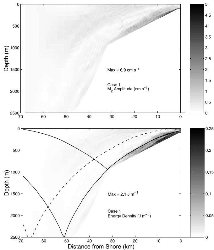
Fig. 8. Along-canyon sections of M2 u amplitude (upper) and energy density, E , (lower) with characteristics emanating from the shelf break (—) and reflecting from the coastal boundary (---).
